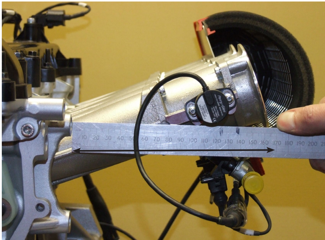
Head to edge of air horn - 170mm Air horn depth - 19mm
