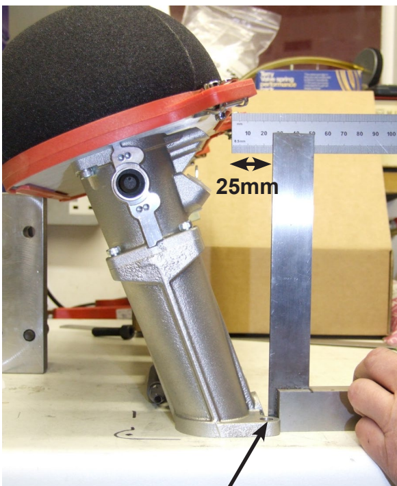
Centre of inlet manifold mounting hole to flat red edge of air filter (excluding fixing lugs)
