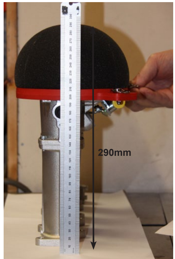
Face of inlet manifold to top of air filter - 290mm
