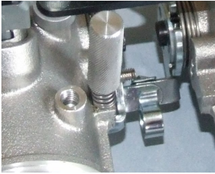
Throttle stop screw
